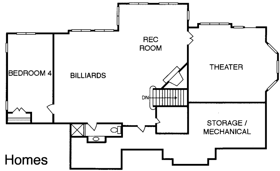
BASEMENT FLOOR
